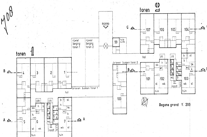
Begane grond 1: 200
