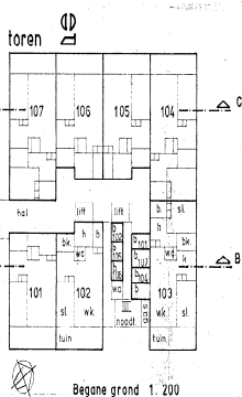
Begane grond 1: 200
