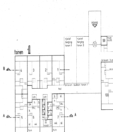
Begane grond 1: 200
