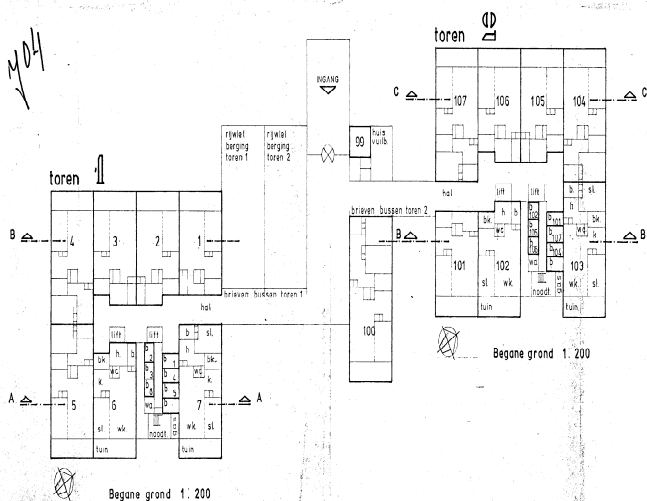
Begane grond 1: 200
